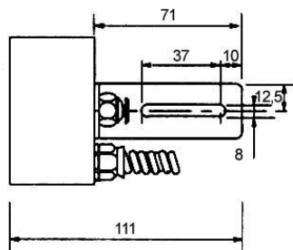
PISTOLET TISP-N
